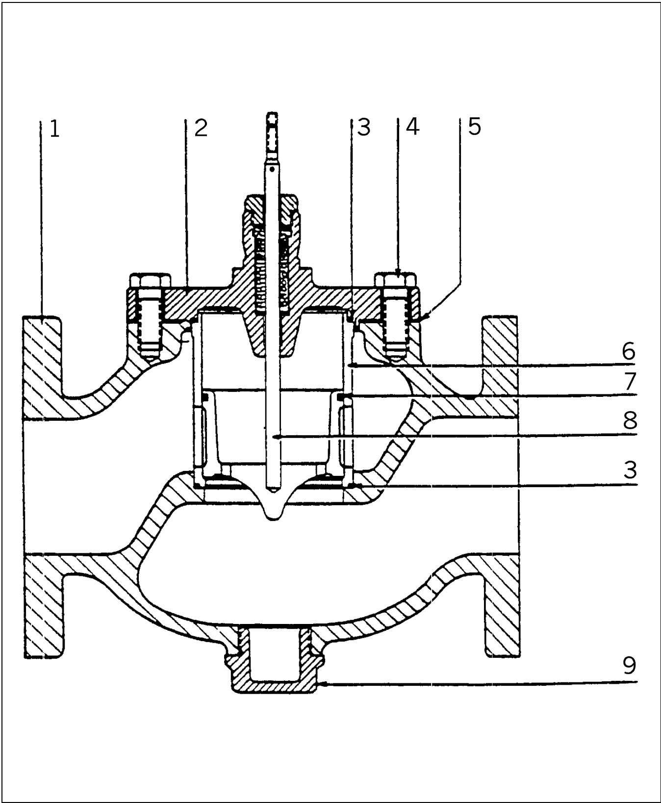
Figure 1 - 2-1/2" - 6" Valves
