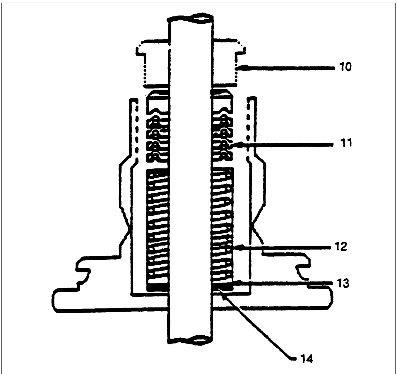
Figure 2 – Teflon V-Ring Packing
