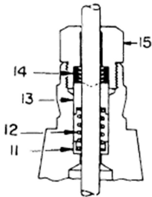
Figure 3. Spring Loaded Teflon Cone Packing.
