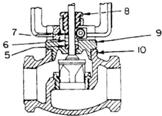
Figure 2 — Teflon Graphite Packing
