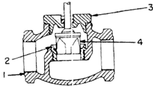
Figure 1. Valve Body, Metal Plug to Metal Seat.
