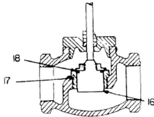
Figure 4. Valve Body, Composition Disc.
